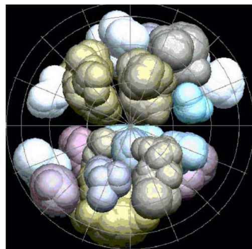
Figure 2. Three-dimensional view of the voids in the IRAS survey. The ZOA, caused by the Galaxy, runs horizontally across the image. The area at the left, near the ZOA with no voids, corresponds to the Great Attractor. The absence of voids from the lower, right-hand part of the image, is due to the Cetus wall and the Perseus-Pisces supercluster.
